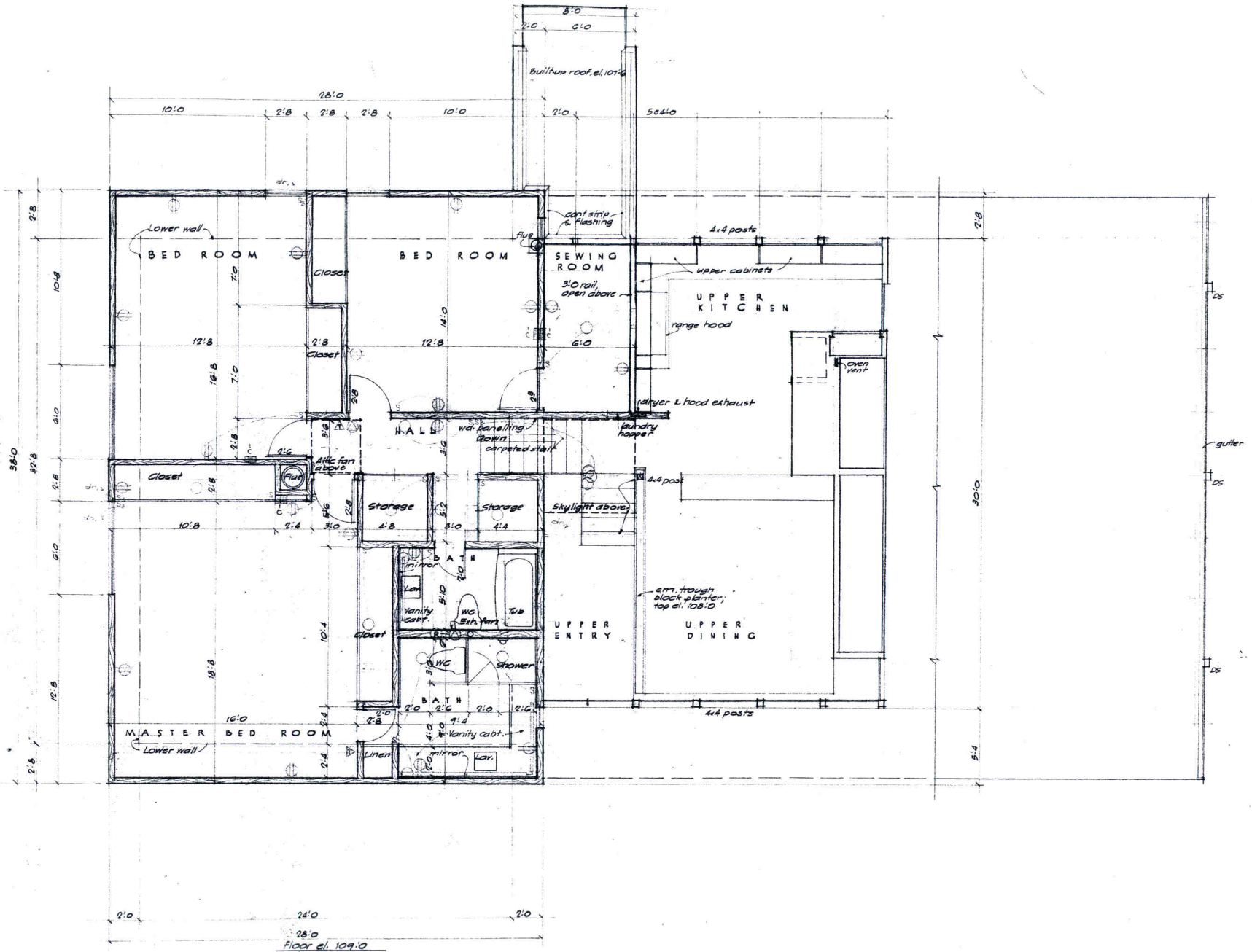
PLAN OF UPPER LEVEL 1/4" = 1'-0"
